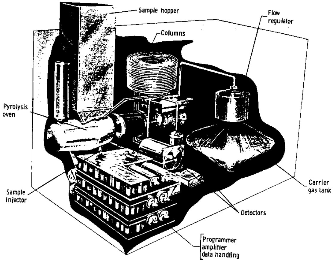
FIGURE 5.—Gas chromatograph.
